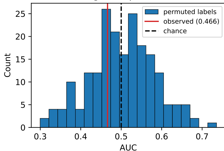
Elastic-net logistic ( p = 0.667 , n = 200 )
