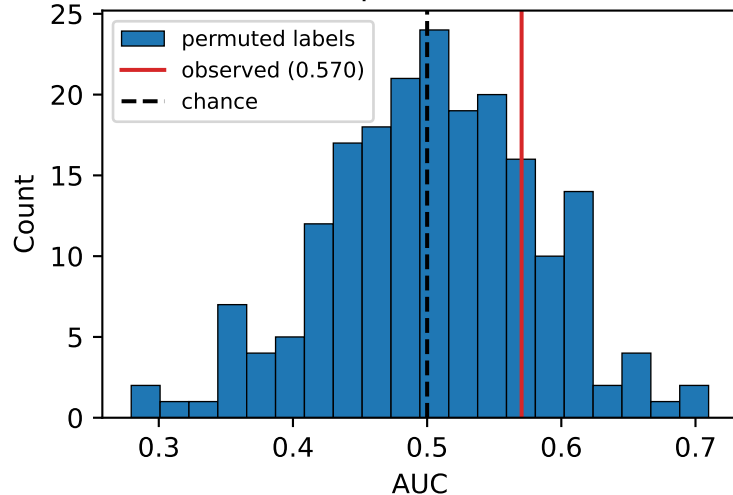
SVM (RBF) ( p = 0.214 , n = 200 )
